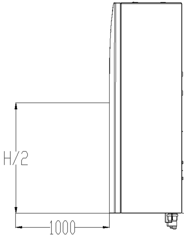
Indoor unit sound pressure level measurement(unit:mm)
