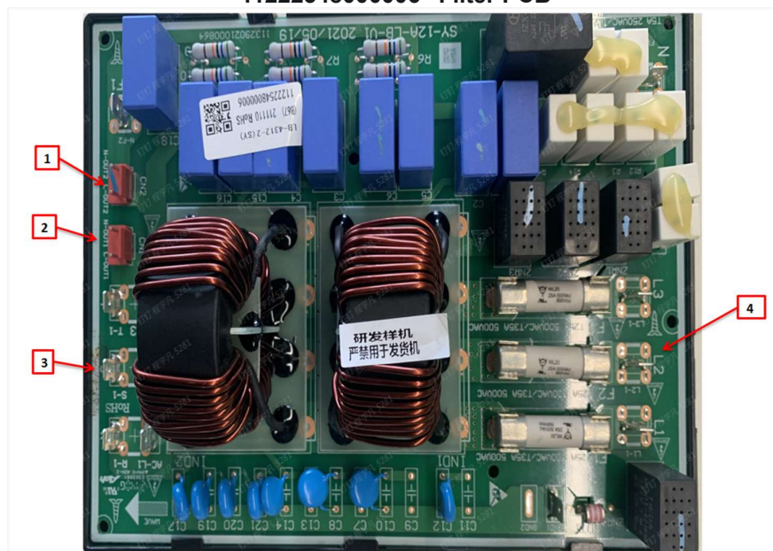
11222548000006 Filter PCB
