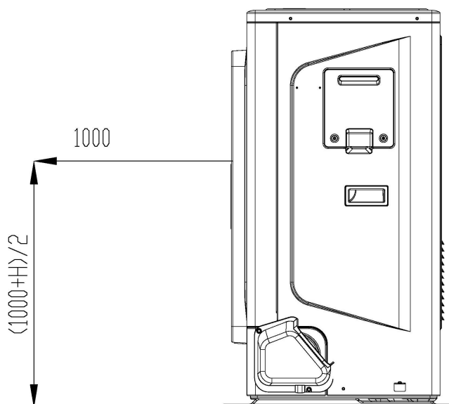
Outdoor unit sound pressure level measurement(unit:mm)
