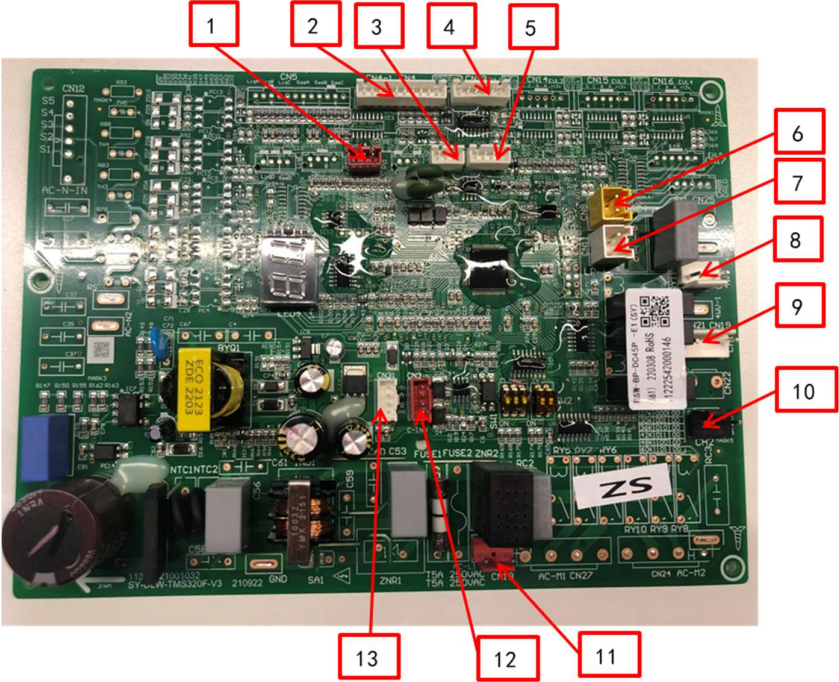
11222542000146 Main PCB
